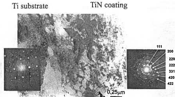
Fig. 5. TEM microstructure of TiN deposited on Ti
