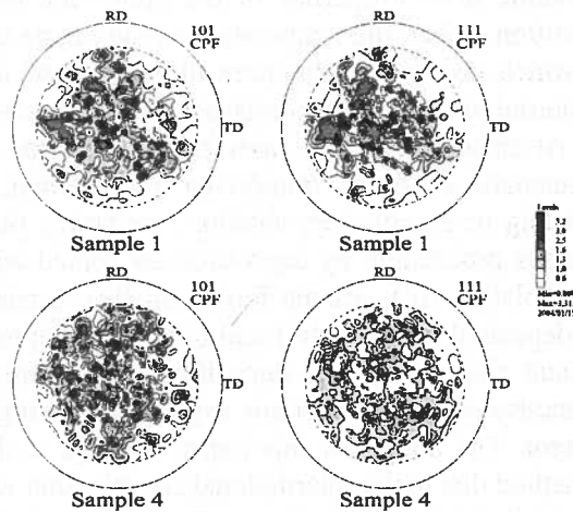
Fig. 2. Pole figure of crystallographic texture measured in the surface layer of titanium alloys subjected to laser remelting in nitrogen atmosphere (nitride phase); (101) pole figure corresponds to Ti_2N tetragonal phase while (111) pole figure corresponds to TiN cubic phase; a) Sample 1 – TiAl1Mn alloy subjected to laser remelting by Nd:YAG laser using overlapping laser tracks; b) Sample 4 – Ti6Al4V alloy subjected to laser remelting by diode laser using individual laser track
