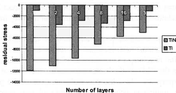
Fig. 8. Residual stress dependence on the number of layers
