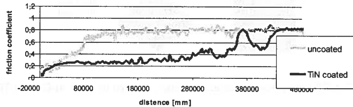
Fig. 9. Friction coefficient variation in the wear test for the Ti/TiN/Ti/TiN system
