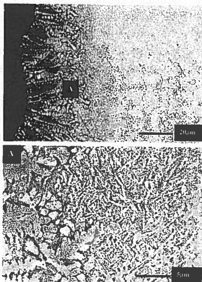
Fig. 1. SEM micrographs of a cross-section of the Ti1Al1Mn alloy subjected to remelting with Nd: YAG laser in nitrogen environment by overlapping laser tracks
