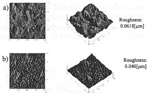
Fig. 7. AFM morphology of surface coatings produced by PLD: a) CrN; b) TiN
