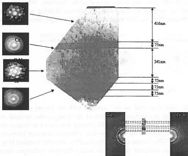
Fig. 6. TEM microstructure of the cross-section coating of the Cr/CrN/Cr/CrCN fabricated by means of PLD method
