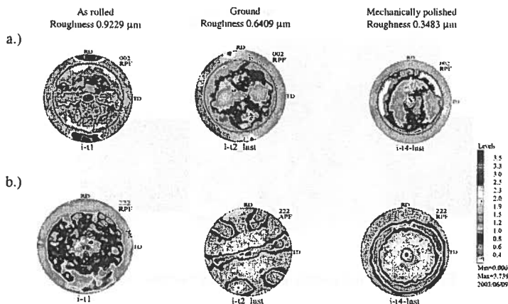
Fig. 3. Pole figures of: a.) titanium substrate; b.) TiN coating
