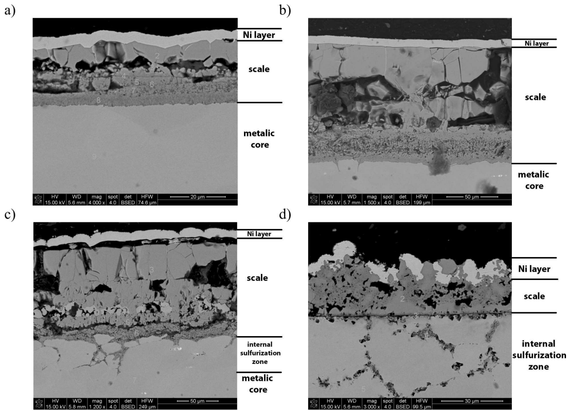
Fig. 6. SEM image showing fracture of Crofer 22APU steel sample sulphurised in H_2/H_2S atmosphere at partial pressure of sulphur vapours 10^{-3} Pa and temperature: a) 600°C, b) 700°C, c) 800°C, d) 900°C
