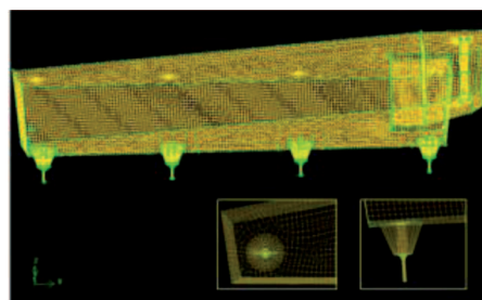
Fig. 1. The computational grid of the tundish geometry of CCM No.2 with the view detail on the computational grid of the tundish nozzle
