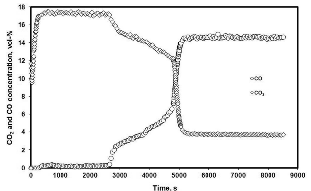
Fig. 6. Dependence of the CO 2 and CO content in the reaction gases on time, for slag no 1 at 1373K in the second stage
