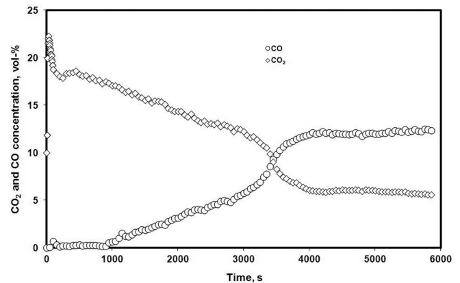
Fig. 8. Concentrations of the \text{CO} and \text{CO}_2 versus time, during the passing of the \text{CO} - \text{CO}_2 mixture (4:1) through slag no 4, at 1373 K
