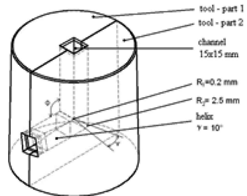
Fig. 3. Insert of the ECAP tool with built-in helix
