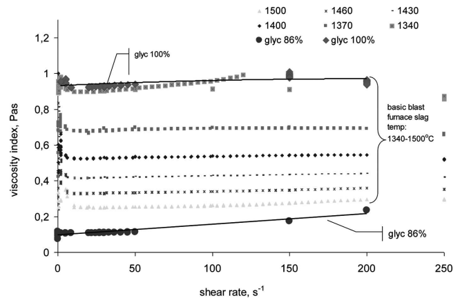
Fig. 3. Viscosity curves for basic blast furnace slag and glycerol solutions
