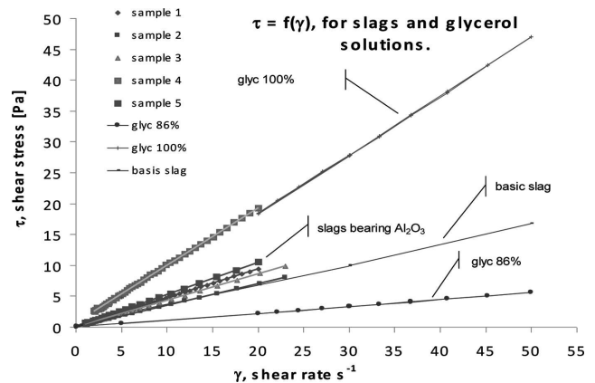
Fig. 4. Flow curves for various rheological liquids
