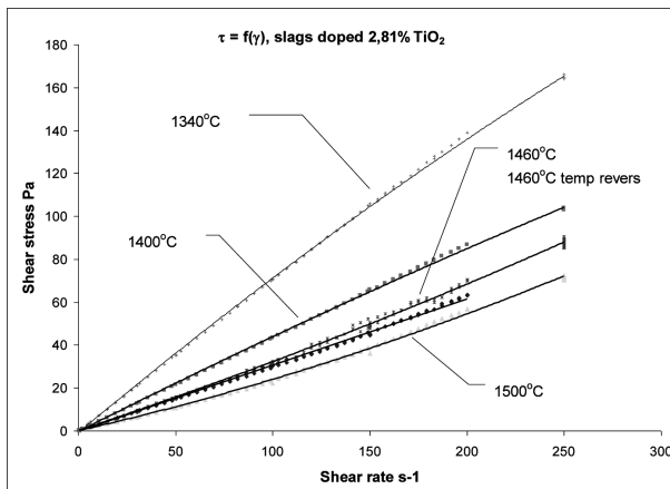
Fig. 8. Flow curves for slags doped with \text{TiO}_2
