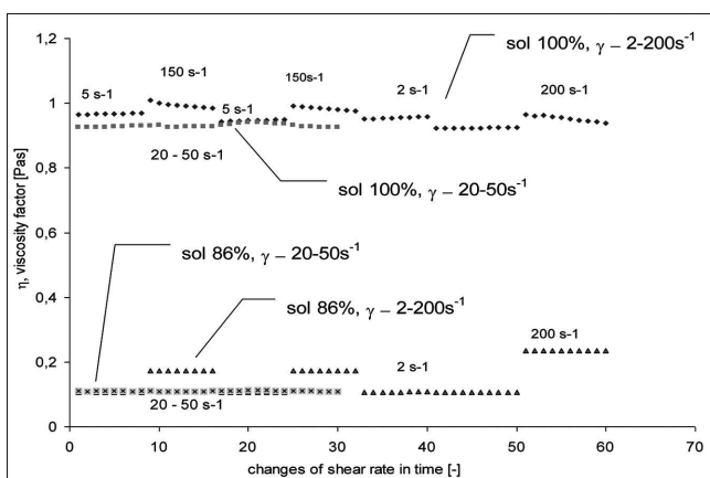
Fig. 9. Viscosity changes in steps (a and b etaps)
