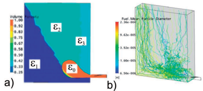
Fig. 2. Solid particles PC trajectories and porosity of the coke bed [18]
