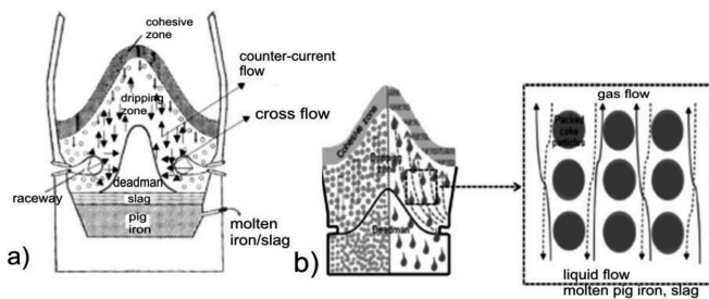
Fig. 1. Blast furnace dripping and cohesive zones [14,15]
