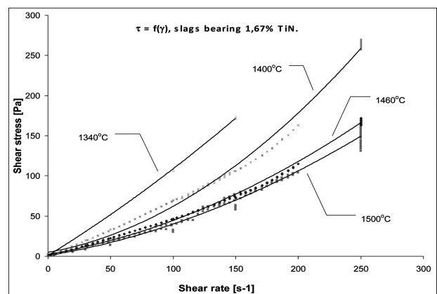
Fig. 7. Flow curves for slags bearing solid particles – TiN
