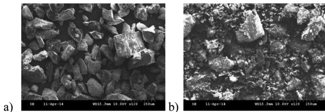
Fig. 5. Solid fine particles for “cold” experiments a) anthracite <90\mu\text{m} , magnification x120, b) pulverised coal – PC, magnification x120
