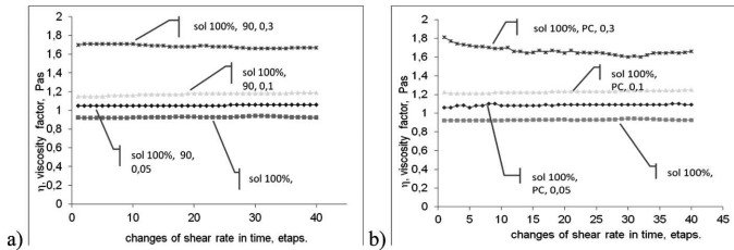
Fig. 11. Relationships between viscosity factors and changes of shear rate in steps
