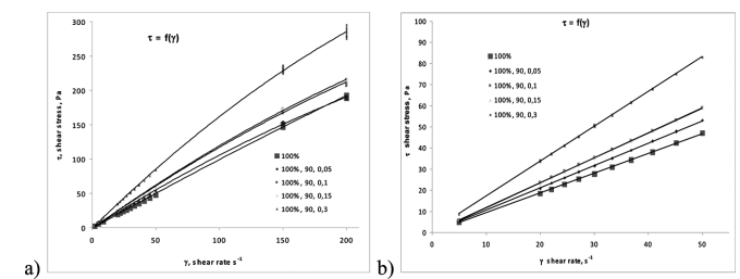
Fig. 10. Flow curves for different shear rate levels; a) up to 200\text{s}^{-1} , b) up to 50\text{s}^{-1}
