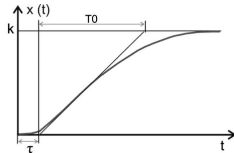
Fig. 5. Typical step response of inert system with delay about transmittance (12) [26]
