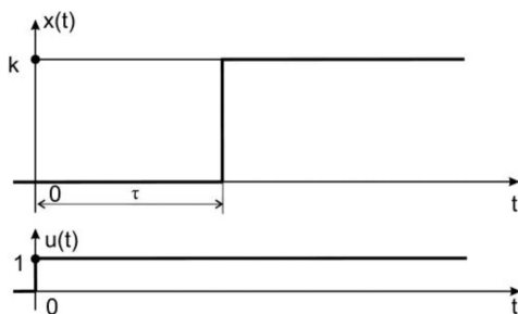
Fig. 4. Step response to the delaying element [26]
