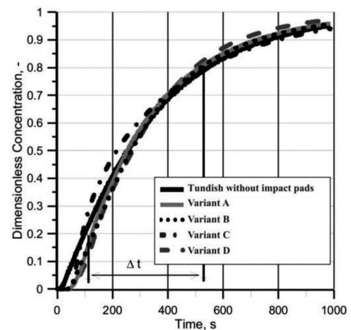
Fig. 2. Example of RTD characteristic – F-type [18]
