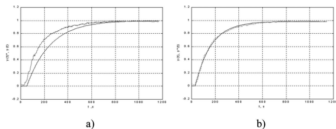
Fig. 6. Example of estimation course: a). measuring results and choice of primary values of time constant, b) estimation results [19]
