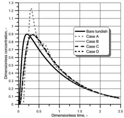
Fig. 1. Example of RTD characteristic – E-type [13]
