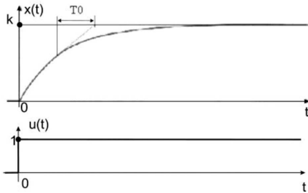
Fig. 3. Output signal of the inert element of 1-st order as a response to the elementary leap of input signal [26]
