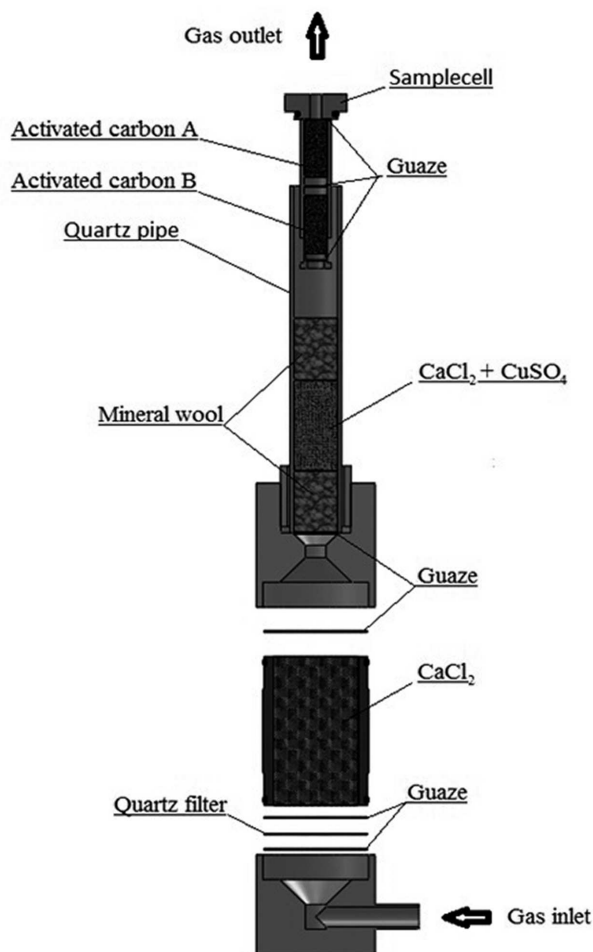
Fig. 2. Capsule for sampling gases for the BTEX content
