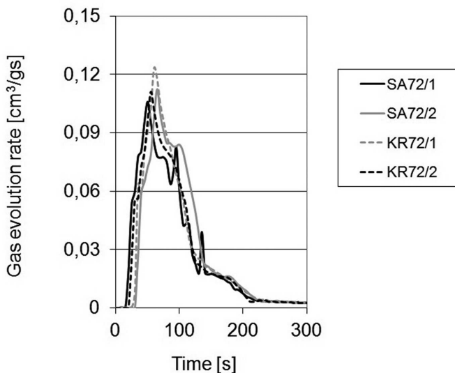
Fig. 4. Velocity of gases emission, from the investigated moulding sands after pouring the mould with cast iron of a temperature of 1350°C
