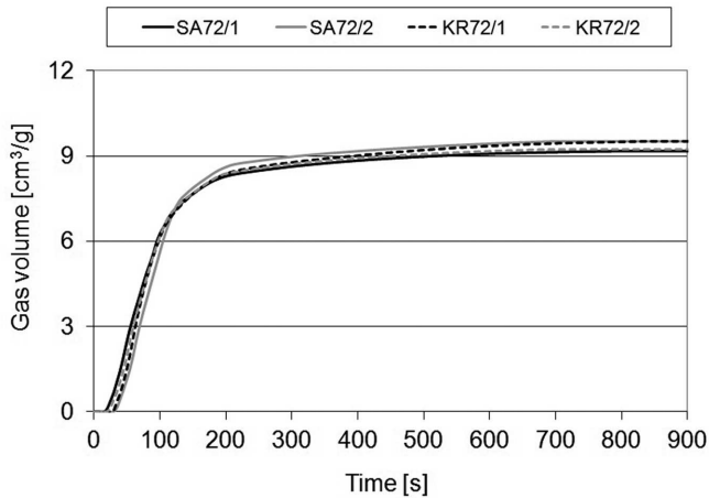
Fig. 3. Emissivity of gases in time, from the investigated moulding sands after pouring the mould with cast iron of a temperature of 1350°C
