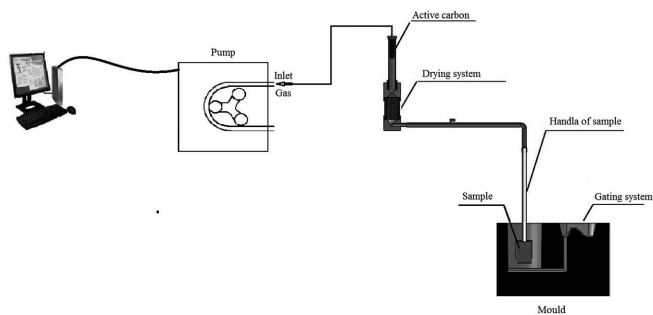
Fig. 1. Experimental stand for the determination of the emitted gases volume and the BTEX emission [11-15]
