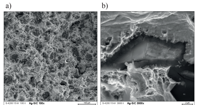
Fig. 3. Ag-matrix composite reinforced with 20 mm SiC particles: a) distribution of the particles in the matrix, b) fracture observed following the tensile test
