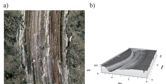
Fig. 8. Wear trace of the Ag- \text{Al}_2\text{O}_3 composite with abrasion-related ploughing (zoom: 50x)
