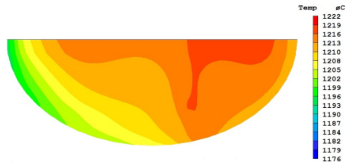
Fig. 4. Slag temperature distribution in the middle of a domain in the system of 3 nozzles in the cross-section
