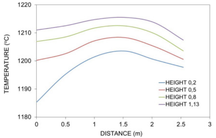
Fig. 9. Course of slag temperature in the system of 3 nozzles in the plane Y=2,3
