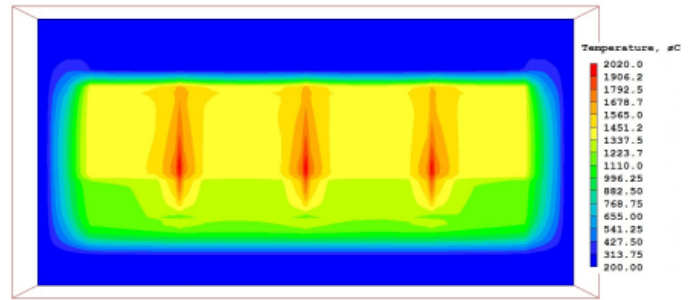
Fig. 3. Temperature distribution in furnace in the area of nozzles
