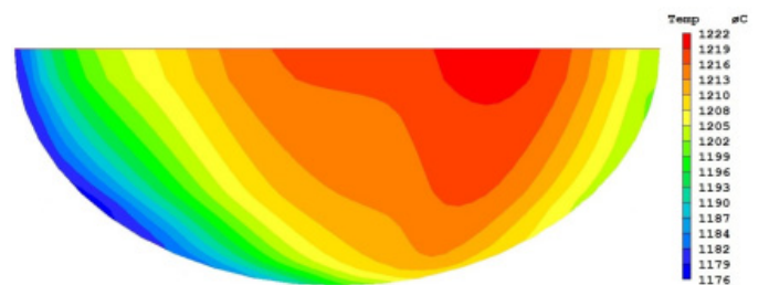
Fig. 5. Slag temperature distribution in the beginning of a domain in the system of 3 nozzles in the cross-section
