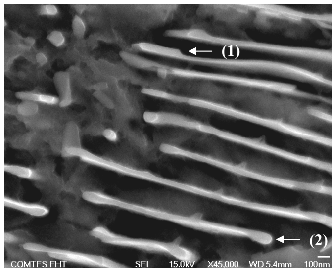
Fig. 2 Regime 800/15q. Dissolution of the cementitic lamellae in progress. Ridges thinning the lamella are formed (1) and thickened edges (2)
