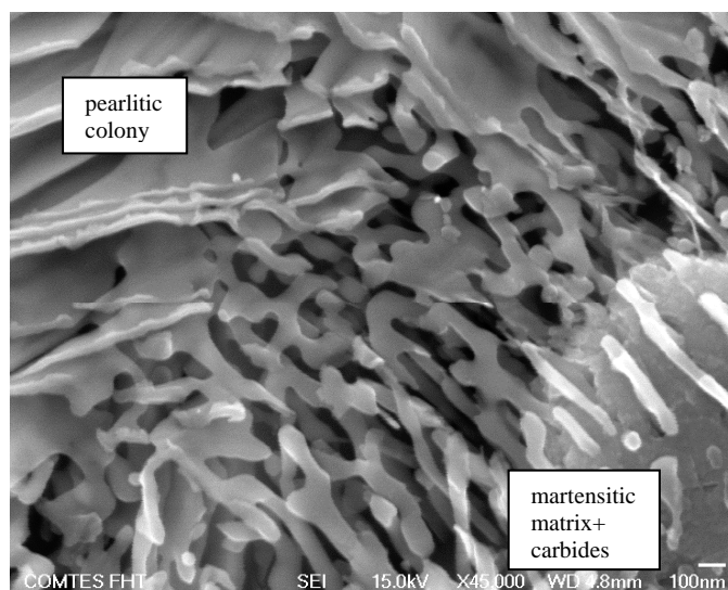
Fig. 3. Fragmentation at the \alpha - \gamma interface. Regime 800q
