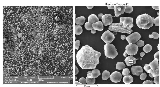
Fig. 3. EDX microscopic analysis of Additive 1
