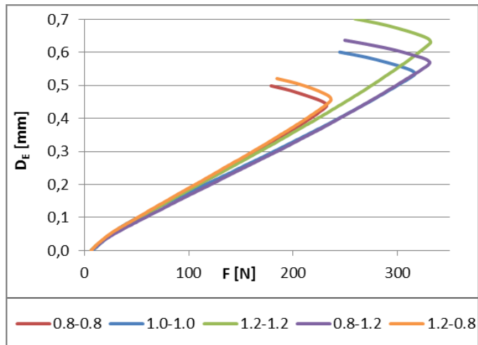
Fig. 2. Elasticity D_E of chosen moulding sands (Table 1) after 24 h of hardening
