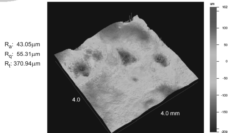
Fig. 8. Example of visualization of the 3D geometry of the surface of sample cut out from the casting made in B type sand mould and the determined surface roughness parameters
