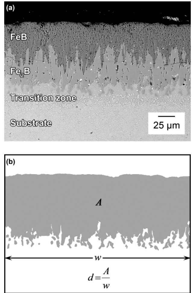
Fig. 1. Schematic showing the measurement procedure for estimating the boride layer thickness (the microstructure shown is that of the specimen borided with Ekabor II powders at 1273 K (1000°C) for 6 h)
