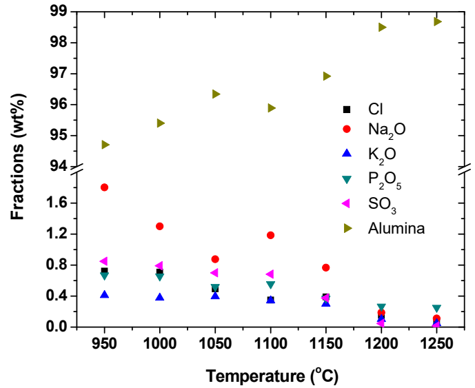
Fig. 7. Fractions of Group II impurities (wt%) in relation to the purity of alumina from calcinated ACH in a step of 50°C from 950 to 1250°C
