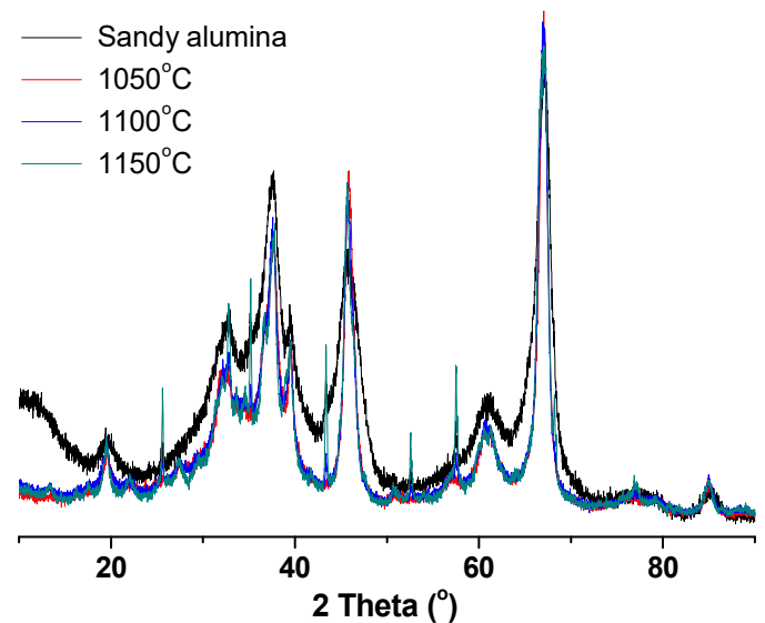
Fig. 8. XRD spectra of sandy alumina by Bayer process and alumina from calcinated ACH at temperatures of 1050, 1100 and 1150°C
