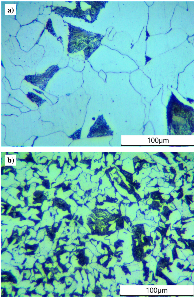
Fig. 1. The microstructure of St3S steel (a) and S235 steel (b), magnification 500×
