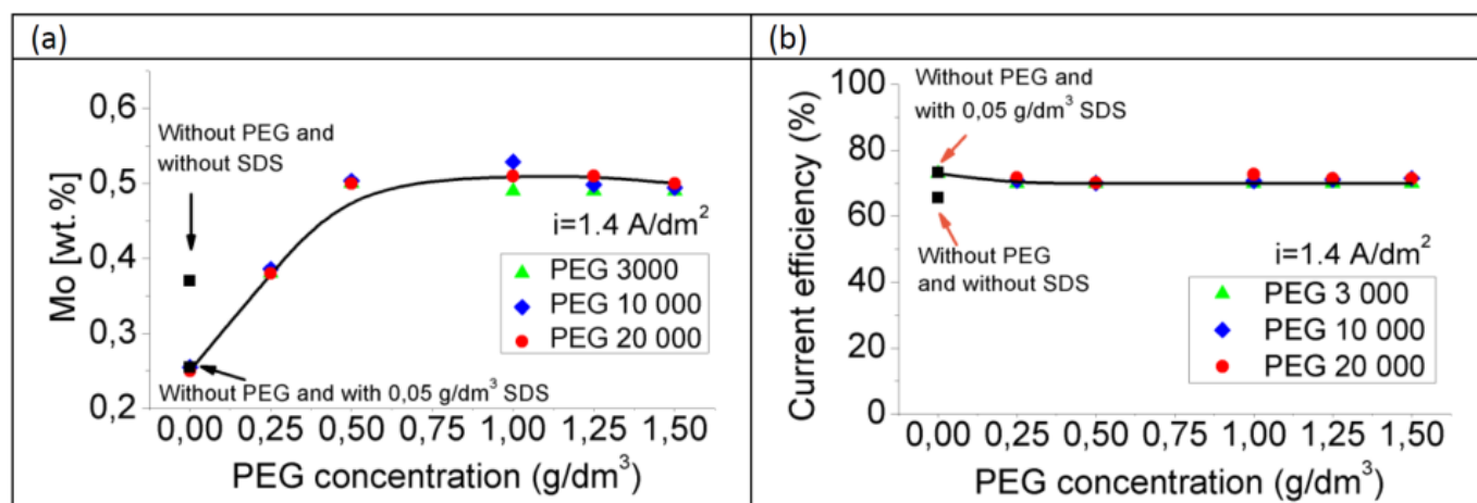
Fig. 1. Effect of polyethylene glycol concentration in electrolyte on the electrodeposition of Zn-Mo layers. (a) Mo content in deposits and (b) current efficiency of the electrodeposition process as a function of polyethylene glycol concentration in electrolyte. Electrodeposition conditions: i = 1.4 \text{ A/dm}^2 , Q = 30 \text{ C} , \omega = 12.6 \text{ rad/s} , and T = 20^\circ\text{C} , Fe substrate
