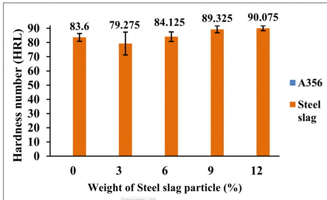
Fig. 2. Hardness of A356/Steel Slag Composites
