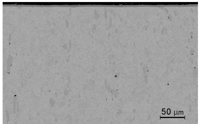
Fig. 5. The SEM image of the X210Cr12 tool steel with the Cr/CrN hybrid coating
