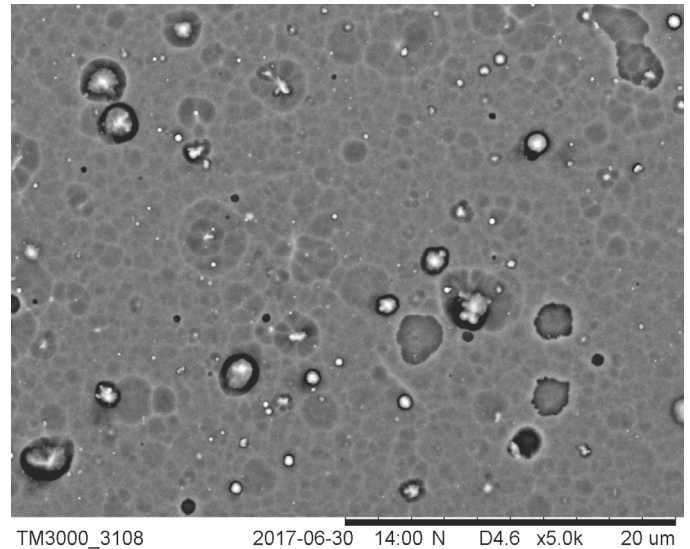
Fig. 4. The SEM image of the surface of the tool steel sample with the Cr/CrN hybrid coating
