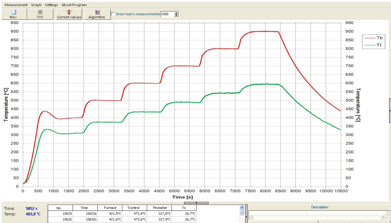
Fig. 8. Temperature changes recorded during measurement
