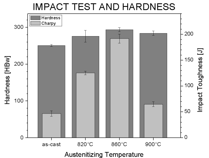
Fig. 4. Brinell hardness and unnotched Charpy test results as a function of austenitizing temperature. The values are an average of the highest three test values of the four tested samples
