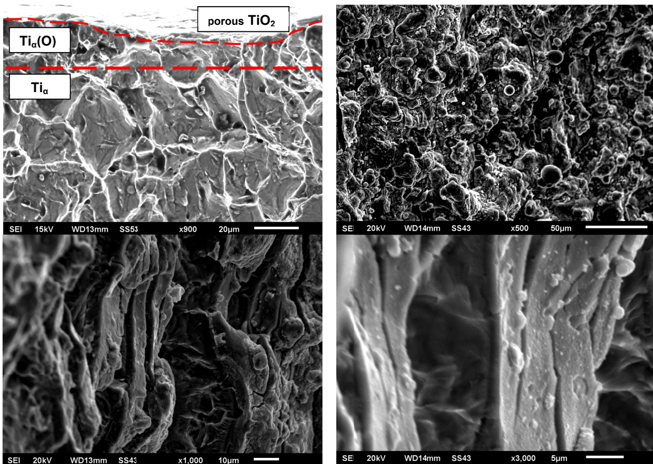
Fig. 1. SEM images of Ti Grade 2 substrate microstructure and fracture after fluidized bed diffusive treatment (FADT) at 640°C/8h
