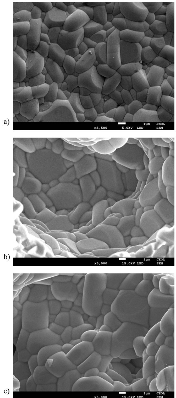
Fig. 1. SEM pictures of \text{BaBi}_2\text{Nb}_2\text{O}_9 ceramics a) without doping b) doped with 1 at. % La c) doped with 5 at. % La
