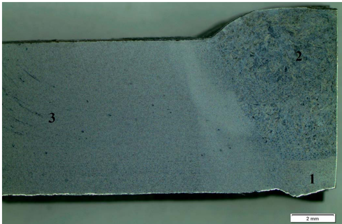
Fig. 1. Macrostructure of an examined joint: 1 – analysed area No. 1; 2 – analysed area No. 2; 3 – a base material – the T91 steel
