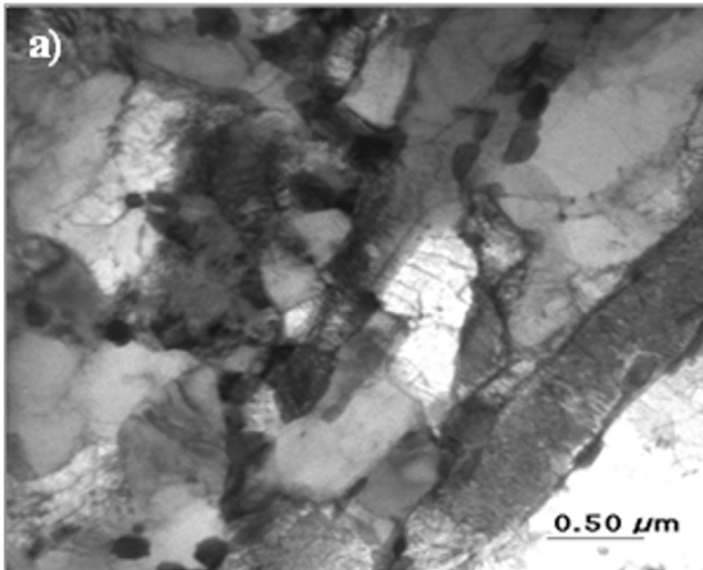
Fig. 3. Microstructure of the base material – the T91 steel, TEM
