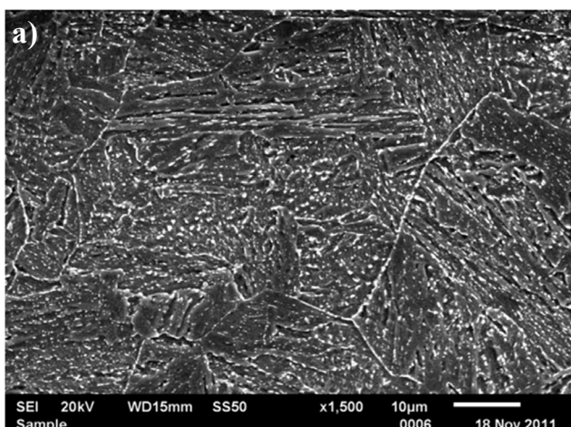
Fig. 4. Microstructure of the weld from the root of the weld, SEM
