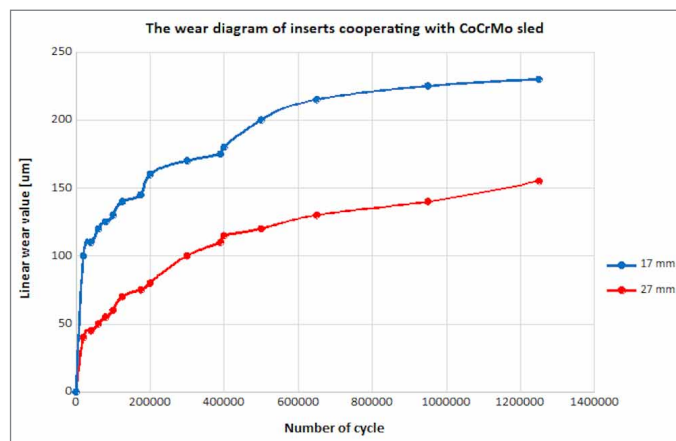
Fig. 12. Influence of load force on linear wear value of the polyethylene insert
