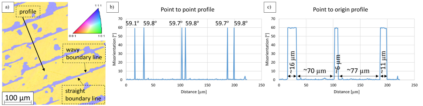
Fig. 5. EBSD map (a) with misorientation point-to-point profile (b) and point-to-origin profile (c) obtained for sample with Co addition
