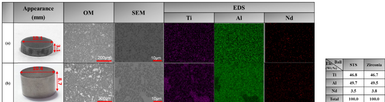
Fig. 5. SEM images and EDS analyses of sintered samples prepared with (a) STS balls and (b) zirconia balls
