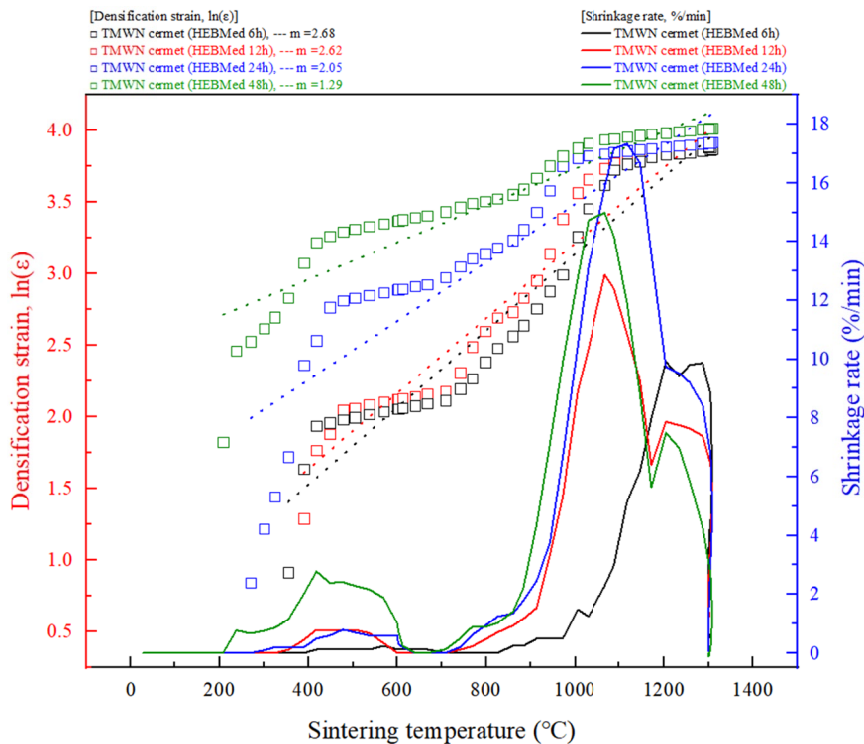
Fig. 1. Densification strain and shrinkage rate as a function of sintering temperature of TMWN cermets
