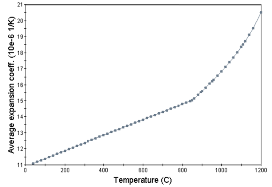
Fig. 10. Relationship between coefficient of thermal expansion and temperature
