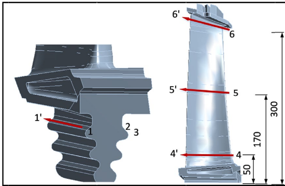
Fig. 16. Analysis paths of the tenon teeth and the blade body
