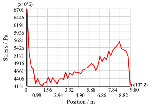
(a) 1-1' position
