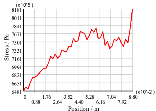
(b) 2-2' position
