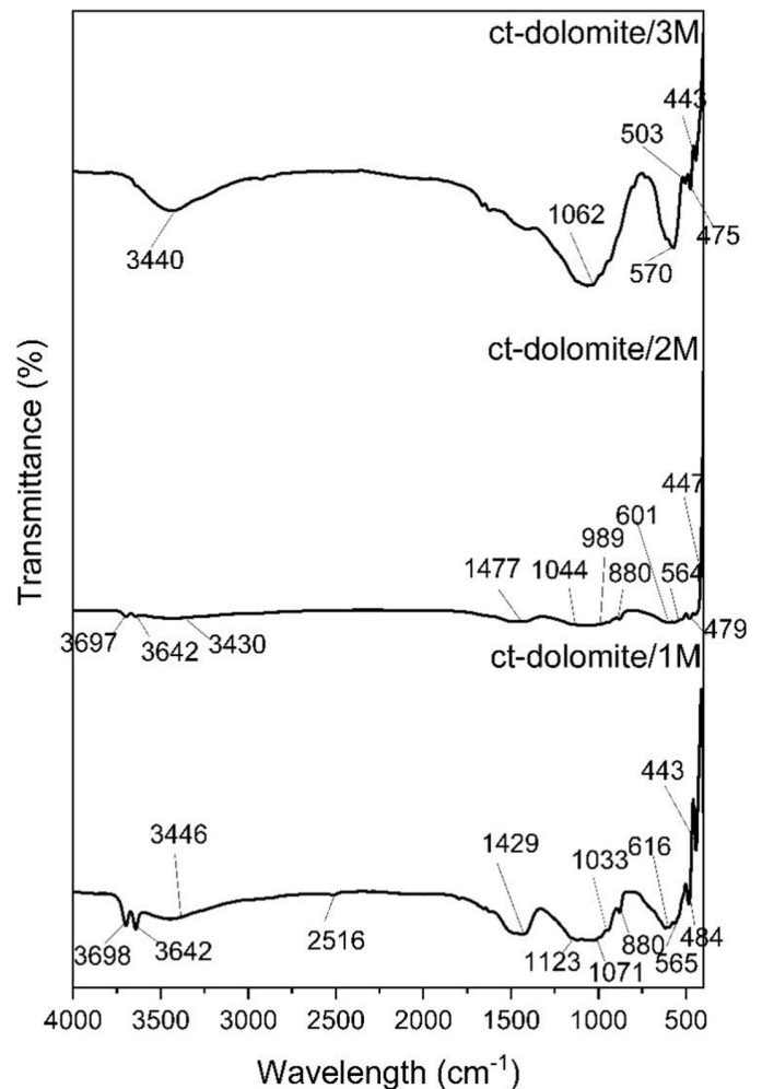
Fig. 2. FTIR spectra of treated-dolomite with various concentration of nitric acid: (a) 1 M; (b) 2 M; and (c) 3 M
