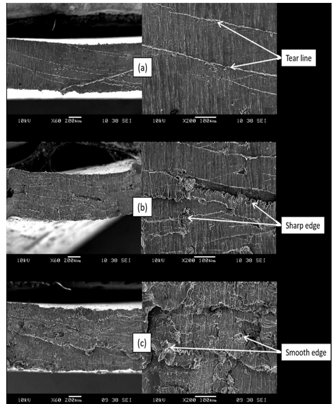
Fig. 4. SEM micrograph of UHMWPE/ct-dolomite composites
