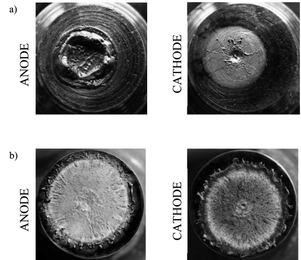
Fig. 15. Macrophotos of contacts surfaces after turning off the 2.5 kA current: a) W-Q = 13.6 C, E = 255 J; b) Ag-W50-Q = 13,7 C, E = 257 J
