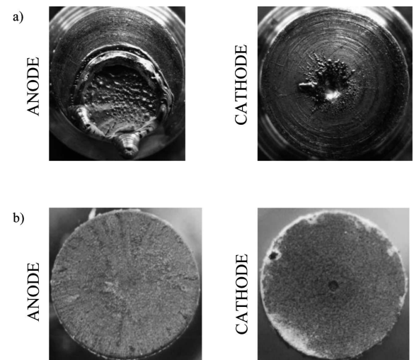
Fig. 16. Macrophotos of contacts surfaces after turning off the 4 kA current: a) W-Q = 20,4 C, E = 408 J; b) Ag-W50-Q = 23,2 C, E = 469 J
