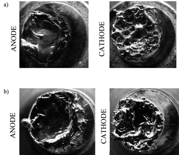
Fig. 14. Macrophotos of contact surfaces after turning off the 2.5 kA current: a) Cu-Q = 12.5 C, E = 306 J; b) Ag-Q = 12.7 C, E = 258 J
