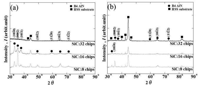
Fig. 2. X-ray diffraction (XRD) pattern of AlN/SiCN composite coating on (a) thin film method and (b) - 2 method
