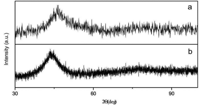
Fig. 1. X-ray diffraction patterns for the investigated alloys: \text{Fe}_{82}\text{Zr}_7\text{Nb}_2\text{Cu}_1\text{B}_8 (a), \text{Fe}_{86}\text{Zr}_4\text{Y}_3\text{Nb}_1\text{Cu}_1\text{B}_5 (b)
