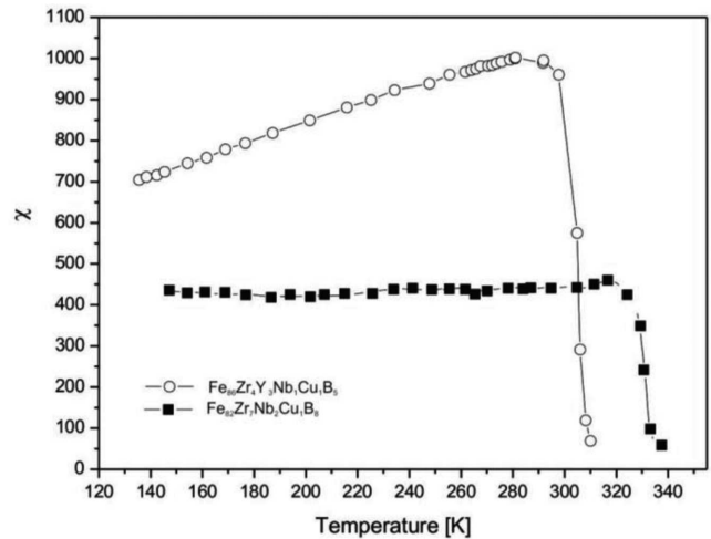
Fig. 4. The magnetic susceptibility curves for the amorphous alloys in the as-quenched state
