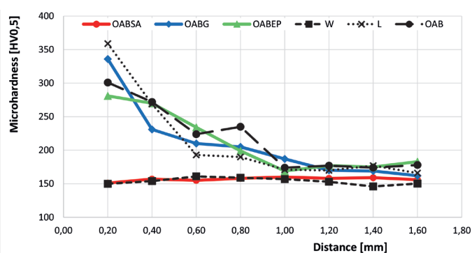
Fig. 4. Results of hardness measurement (HV0,5) on the side surface of links in direction from cutting edge to the sample core, black lines – the previous results, colour lines – the current results (W – water jet, L – laser)
