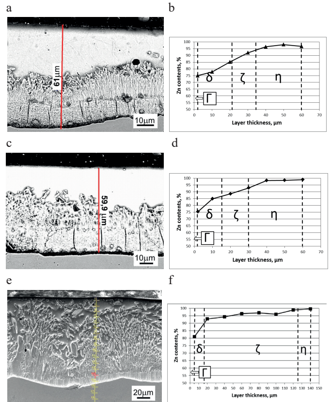
Fig. 7. The Zn coating cross section after OAB cutting and additional treatment and Zn distribution at the coating cross section after OAB cutting and additional treatment (a, b - grinding, c, d – electro-polishing, e, f - softening annealing)
