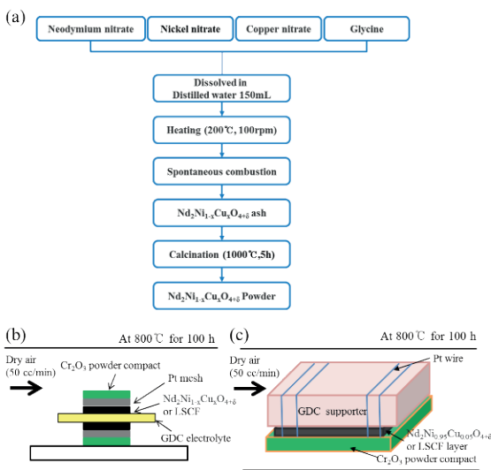
Fig. 1. Schematic diagram for the synthesis of the Nd 2 Ni 1-x Cu x O 4+δ powders (a), the Cr-poisoning experimental (b), and the schematic figure of the samples for conductivity measurement in the gaseous chromium species.
