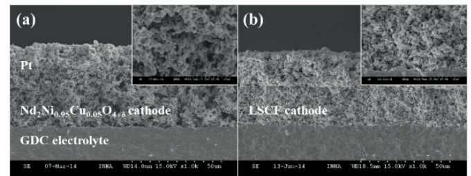
Fig. 3. Cross-sectional SEM images of Nd 2 Ni 0.95 Cu 0.05 O 4+δ /GDC/LSCF symmetric cells
