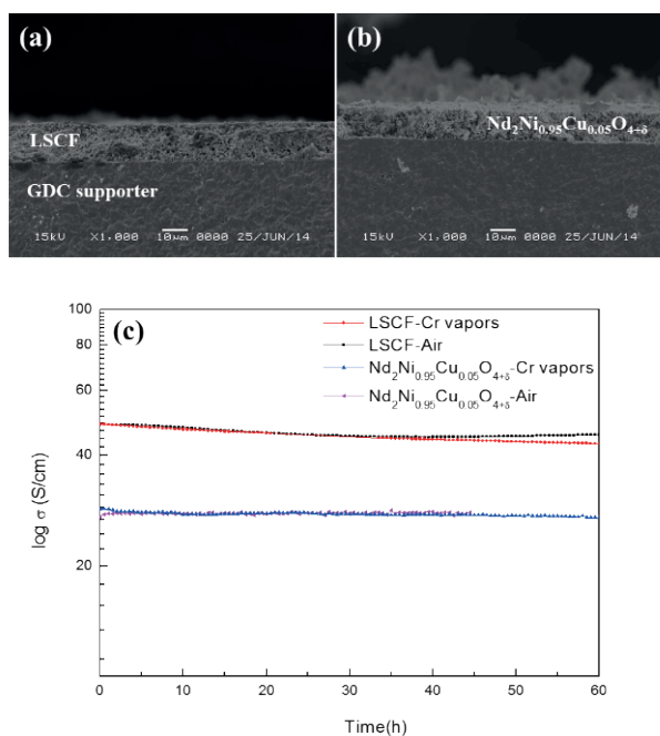
Fig. 5. Electrical conductivity as a function of time of the \text{Nd}_2\text{Ni}_{0.95}\text{Cu}_{0.05}\text{O}_{4+\delta} and LSCF samples in the gaseous chromium species at 800^\circ\text{C}
