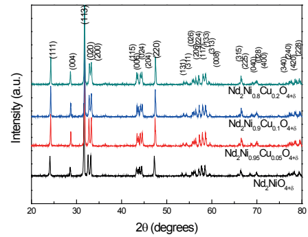
Fig. 2. XRD patterns of the synthesized Nd 2 Ni 1-x Cu x O 4+δ (x=0, 0.05, 0.1, 0.2) powder calcined at 1000°C
