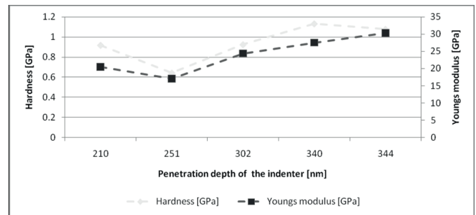
Fig. 13. Nanohardness and Young's modulus of the chitosan coating on Ti-13Nb-13Zr alloy measured for different penetration depths of the indenter
