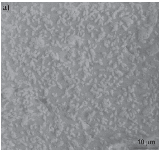
Fig. 10. Surface topography of chitosan coating on near-β Ti-13Nb-13Zr alloy deposited from solution of chitosan (2 g/l) in a mixture of distilled water and 0.5 vol. % of acetic acid as well as 50 vol. % of ethanol stirred for 24 hours (a) and 72 hours (b), AFM
