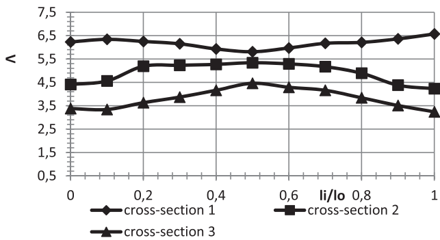
Fig. 7. Distribution \Delta by longitudinal cross section of preform during cogging in flat dies with relative feed 0,6 (cross-section 1 - D_i/D_0 = 0.9 ; cross section 2 - D_i/D_0 = 0.75 ; cross section 3 - D_i/D_0 = 0.5 ; l_i and D_i - the distance to investigated point by length and diameter; l_0 and D_0 - length and diameter of the deformation zone, respectively)
