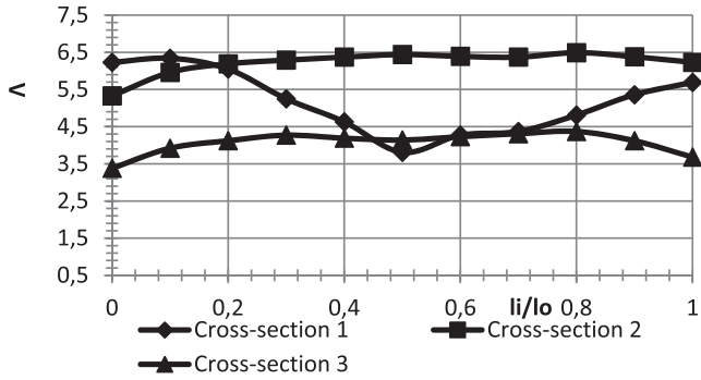
Fig. 6. Distribution \Delta by longitudinal cross section of preform during cogging in flat dies with relative feed 0,8 (cross-section 1 - D_i/D_0 = 0.9 ; cross section 2 - D_i/D_0 = 0.75 ; cross section 3 - D_i/D_0 = 0.5 ; l_i and D_i - the distance to investigated point by length and diameter; l_0 and D_0 - length and diameter of the deformation zone, respectively)
