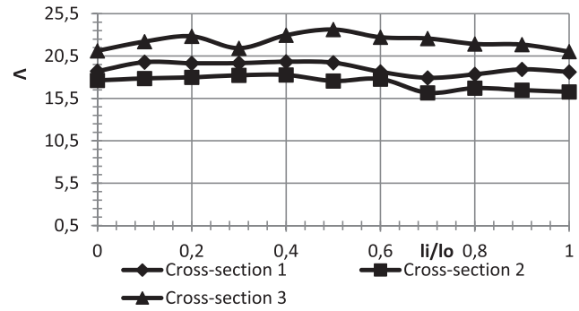
Fig. 8. Distribution \Delta by longitudinal cross section of the preform during cogging in flat dies with relative feed of 1.0 in the first stage, the second stage of 0.8 and 0.6 in the third stage of cogging (cross-section 1 - D_i/D_0 = 0.9 ; cross-section 2 - D_i/D_0 = 0.75 ; cross-section 3 - D_i/D_0 = 0.5 ; l_i and D_i - the distance to investigated point by length and diameter; l_0 and D_0 - length and diameter of the deformation zone, respectively)
