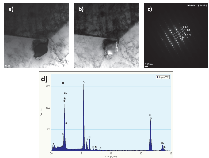
Fig. 2. Microstructure observed with TEM in HR3C steel in the as-received condition: a) bright field, b) dark field, c) diffractogram of NbCrN phase, d) EDS spectrum for NbCrN phase.
