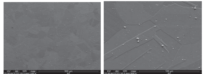
Fig. 1. Microstructure of HR3C steel in the as-received condition, hardness 179 HV10
