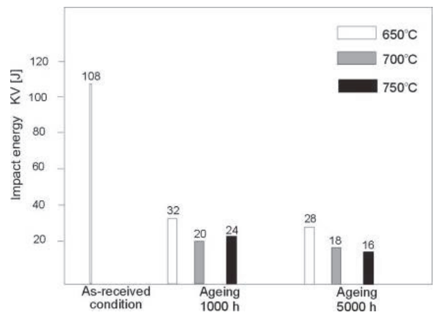
Fig. 9. Effect of time and temperature on impact strength of HR3C steel
