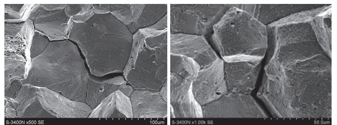
Fig. 10. Brittle intergranular fracture of impact test pieces from HR3C steel after ageing at 650 °C/1,000 h
