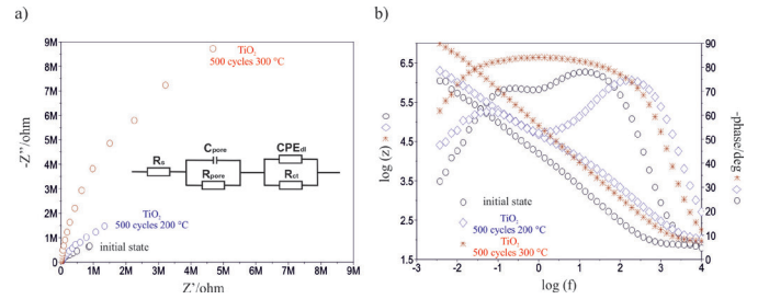
Fig. 3. Impedance spectra for AISI 316LVM steel (initial state, \text{TiO}_2 layer): a) Nyquist diagram, b) Bode diagram
