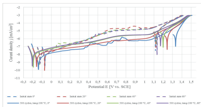
Fig. 1. Curves of polarization of samples after different surface modification
