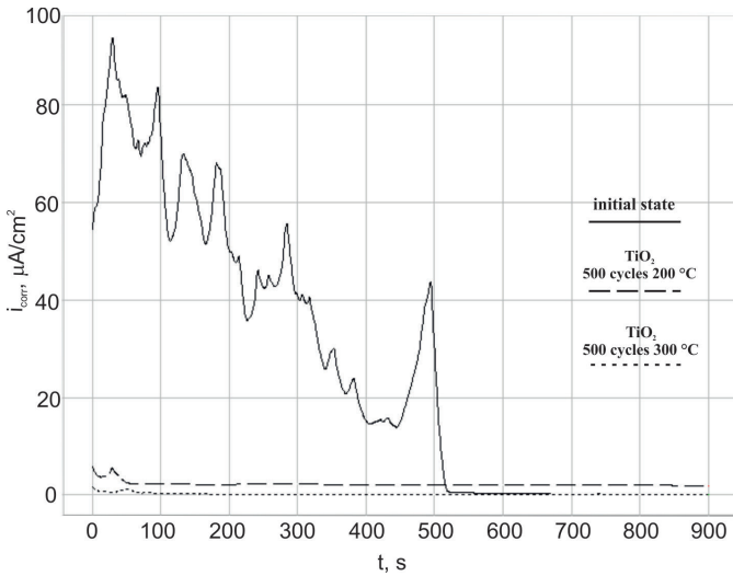
Fig. 2. Exemplary curves of current density in function of time for the initial state, with the \text{TiO}_2 layer 200°C and 300°C samples
