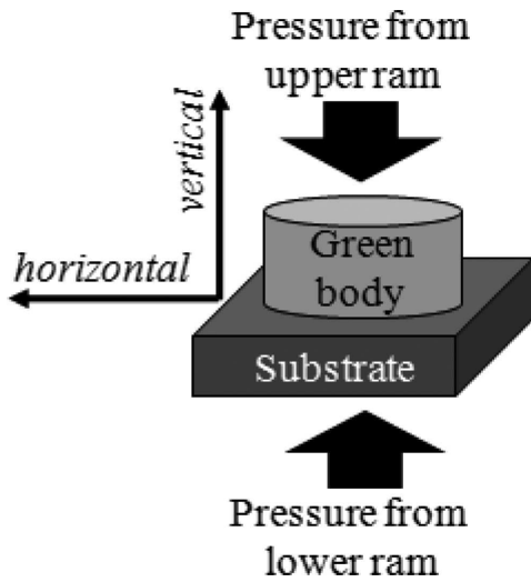
Fig. 1. Schematic illustration of the ITO green body setup for sintering under uniaxial pressure in an open condition
