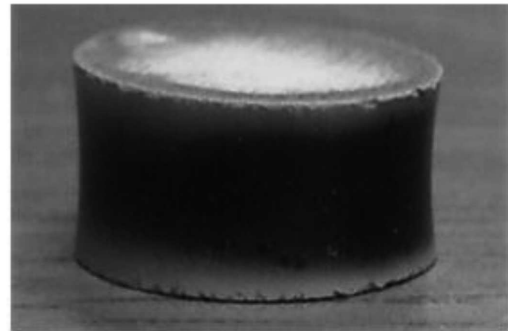
Fig. 7. ITO green body sintered at 1300°C for 2 h under the 0.296 MPa
