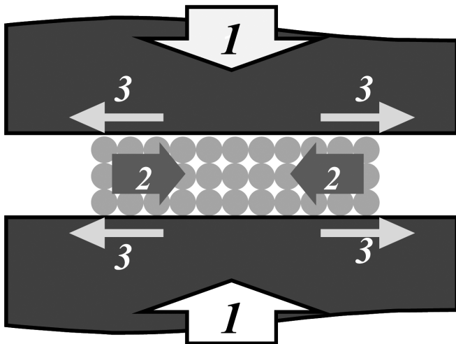
Fig. 6. Schematic illustration of forces acting on the specimen during the joining: Arrow 1 denotes the uniaxial pressure from upper and lower rams, arrow 2 shows the sintering stress of powder compact, and arrow 3 represents the friction force by the rams
