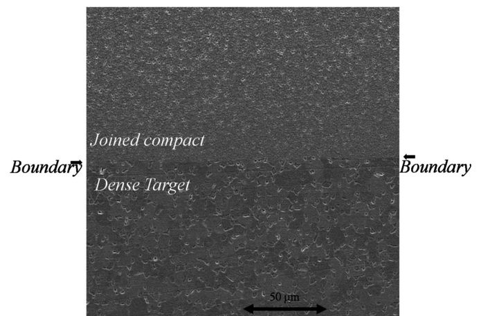
Fig. 5. Boundary between ITO green body and dense target joined by sintering at 1300°C for 2 h under 0.296 MPa
