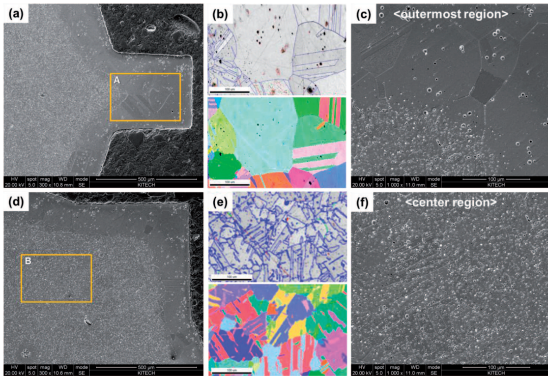
Fig. 6. Microstructures of representative micro feature sintered at 1350°C for 3hrs in 5 torr Ar atmosphere using 4µm powder feedstock. (a), (b) and (c) are SEM and EBSD images at the outermost layer and (d), (e) and (f) are those in the center region
