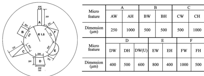
Fig. 2. Schematic drawing of mold cavity and dimension of micro features
