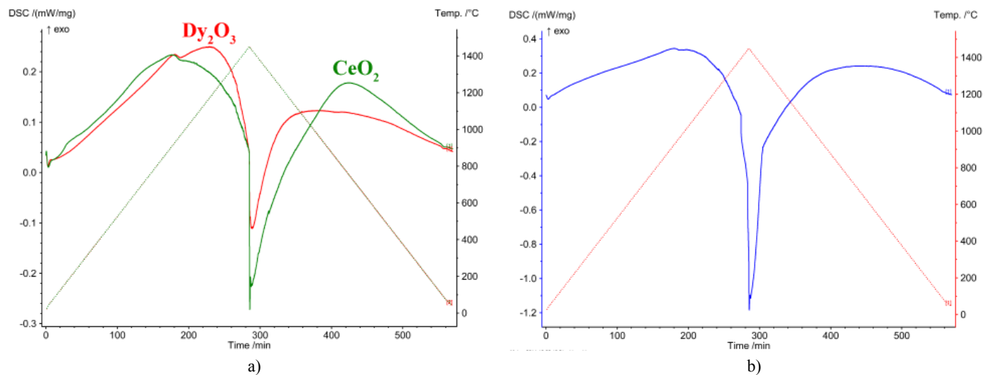
Fig. 1. DSC curves: \text{Dy}_2\text{O}_3 and \text{CeO}_2 (a) and their mixture after milling (b)
