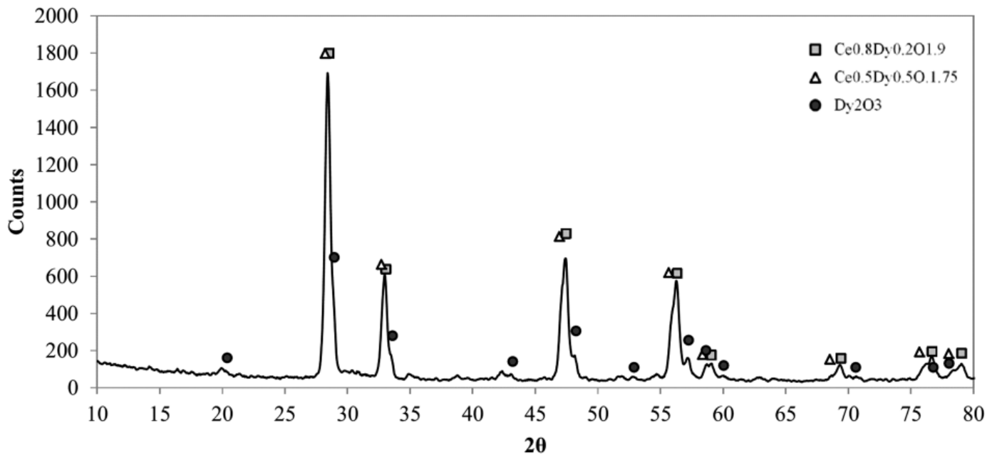
Fig. 5. XRD results of Dy_2O_3 - CeO_2 sintered pellets
