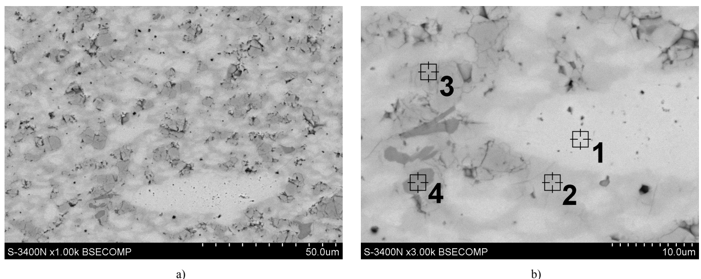
Fig. 2. Microstructure of \text{Dy}_2\text{O}_3 - \text{CeO}_2 sintered pellets with marked spots for EDS analysis
