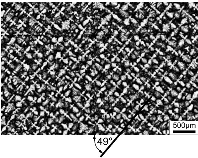
Fig. 4. Micro SEM image example (BSE technique) of the blade root dendritic structure in the area of selector extension along the main blade axis
