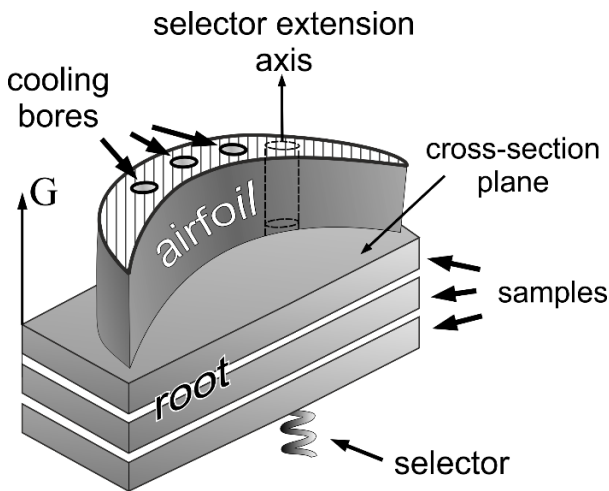
Fig. 1. The shape of the cored turbine blade fragment with a scheme of the sample cutting method. G – the main axis of the blade
