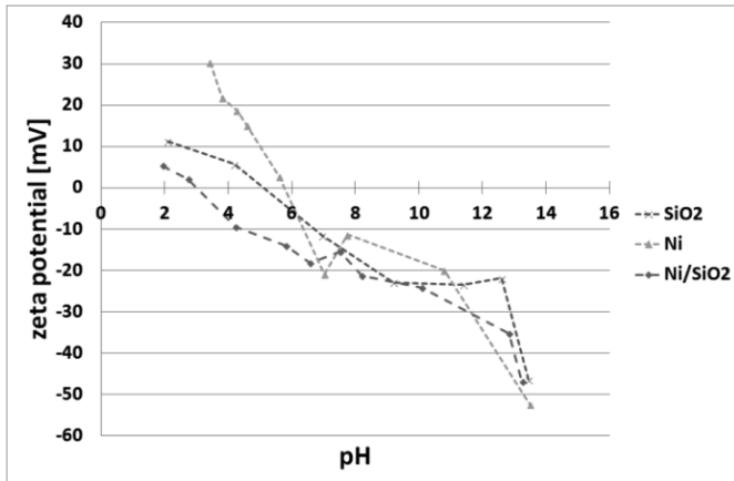
Fig. 1. Relationship between zeta potential and pH for suspensions of \text{SiO}_2 , Ni as well as both \text{SiO}_2 and Ni particles in ethanol
