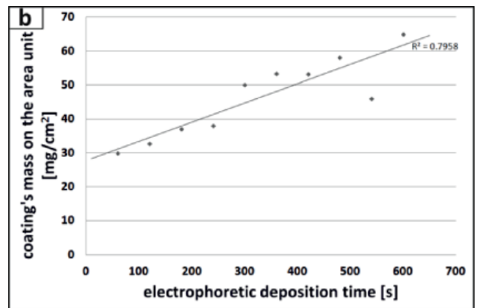
Fig. 3. Relationship between \text{SiO}_2 (a) and Ni/ \text{SiO}_2 (b) coating's mass on the area unit and electrophoretic deposition time
