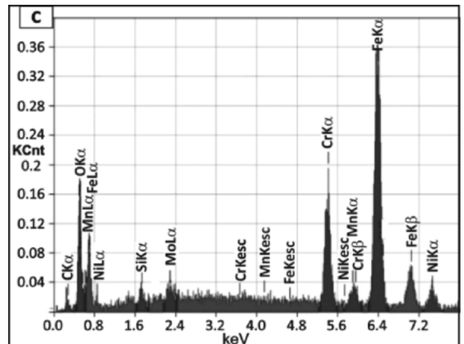
Fig. 5. a) SEM image of the cross-section of SiO 2 coating on X2CrNiMo17-12-2 steel and EDS spectra from SiO 2 coating (b) and Cr 2 O 3 oxide layer (c)
