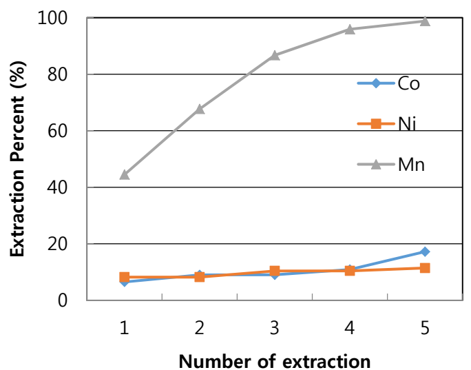
Fig. 3. Changes in extraction of Co, Ni and Mn with the number of extraction experiments
