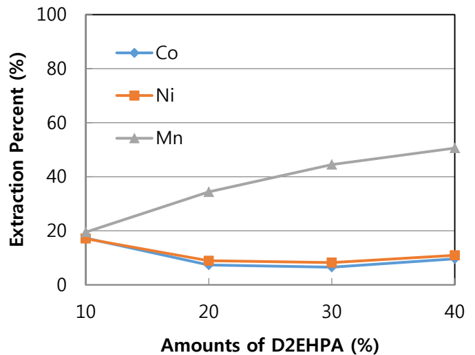
Fig. 1. Changes in extraction of Co, Ni and Mn with varying the amount of D2EHPA
