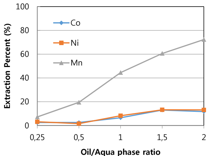
Fig. 2. Changes in extraction of Co, Ni and Mn with the ratio of organic and water volume
