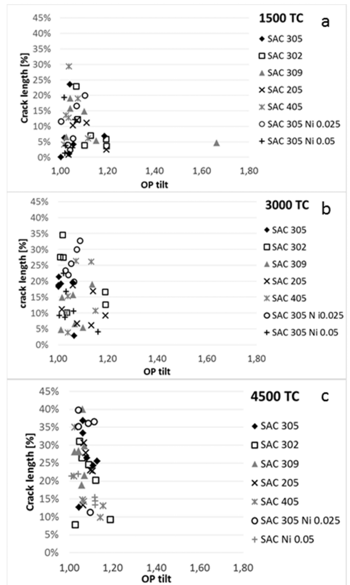
Fig. 4. Measured crack length vs off-plane tilt of THT solder joints a) after 1500 TC, b) 3000 TC, c) 4500 TC
