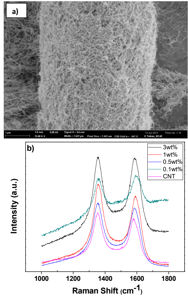
Fig. 1. a) SEM figure of MWCNT powder and b) Raman spectroscopy of as received CNT and after ultrasonication
