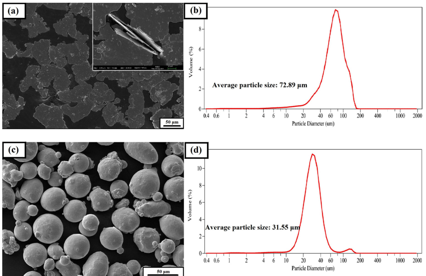
Fig. 1. The FE-SEM images and PSD analyses of (a) and (b) the as-received non-spherical, and (c) and (d) spherical powders, respectively
