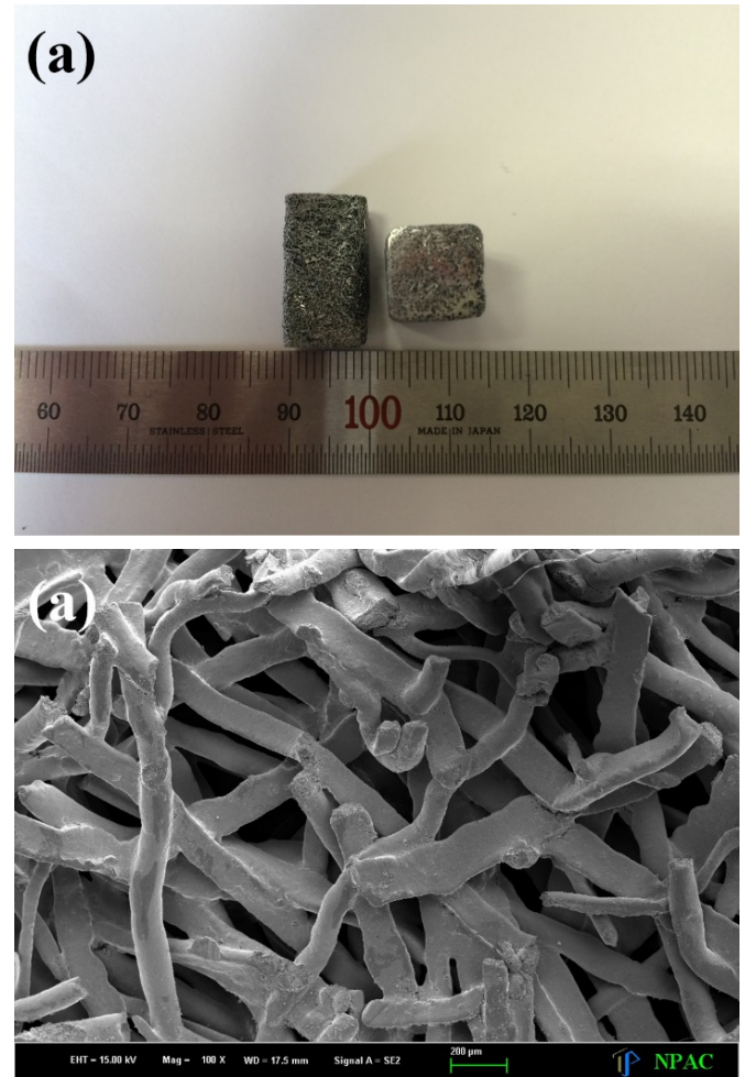
Fig. 3. (a) Optical and (b) SEM image of porous 77Ti-18Nb-5Mo scaffolds
