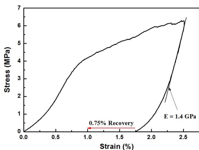
Fig. 5. Compressive strain-stress curve of porous 77Ti-18Nb-5Mo scaffolds
