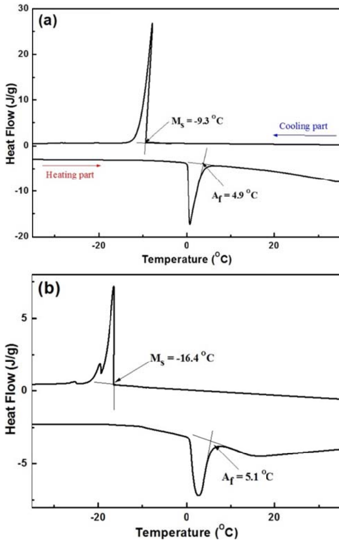
Fig. 2. DSC curves of (a) as-solidified fibers and (b) sintered scaffolds of 77Ti-18Nb-5Mo shape memory alloy
