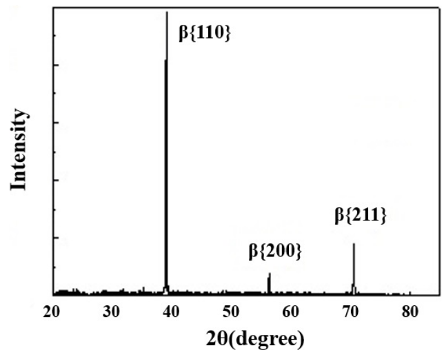
Fig. 4. XRD pattern of porous 77Ti-18Nb-5Mo scaffolds
