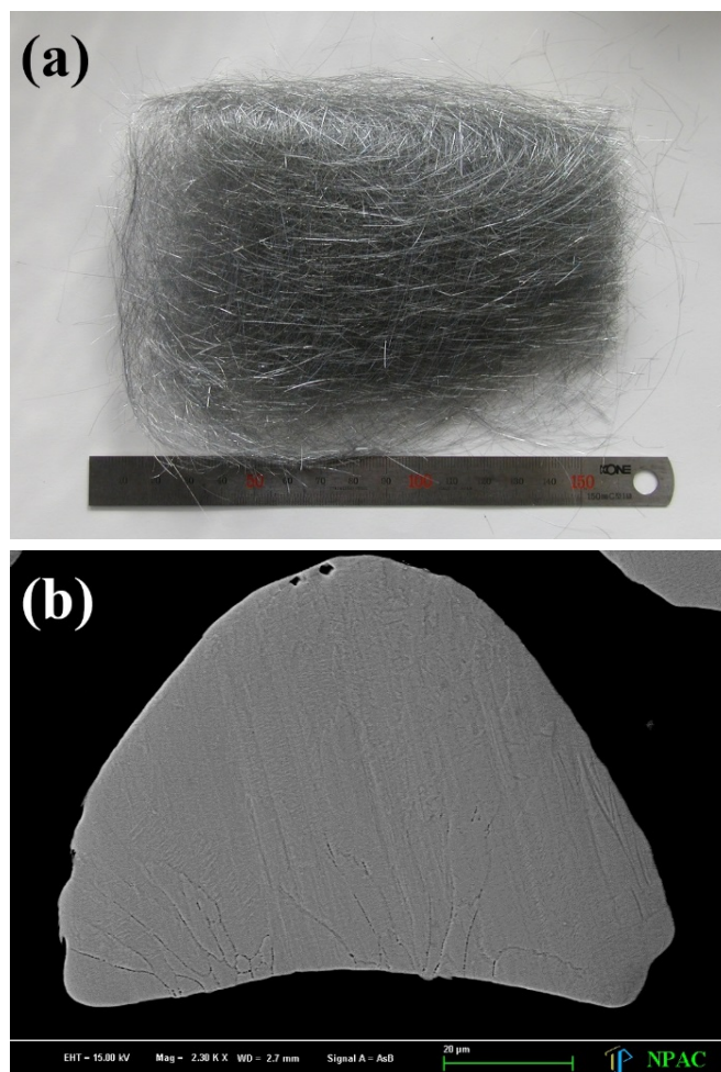
Fig. 1. (a) Photograph and (b) SEM micrograph of etched cross-section of as-solidified 77Ti-18Nb-5Mo fibers
